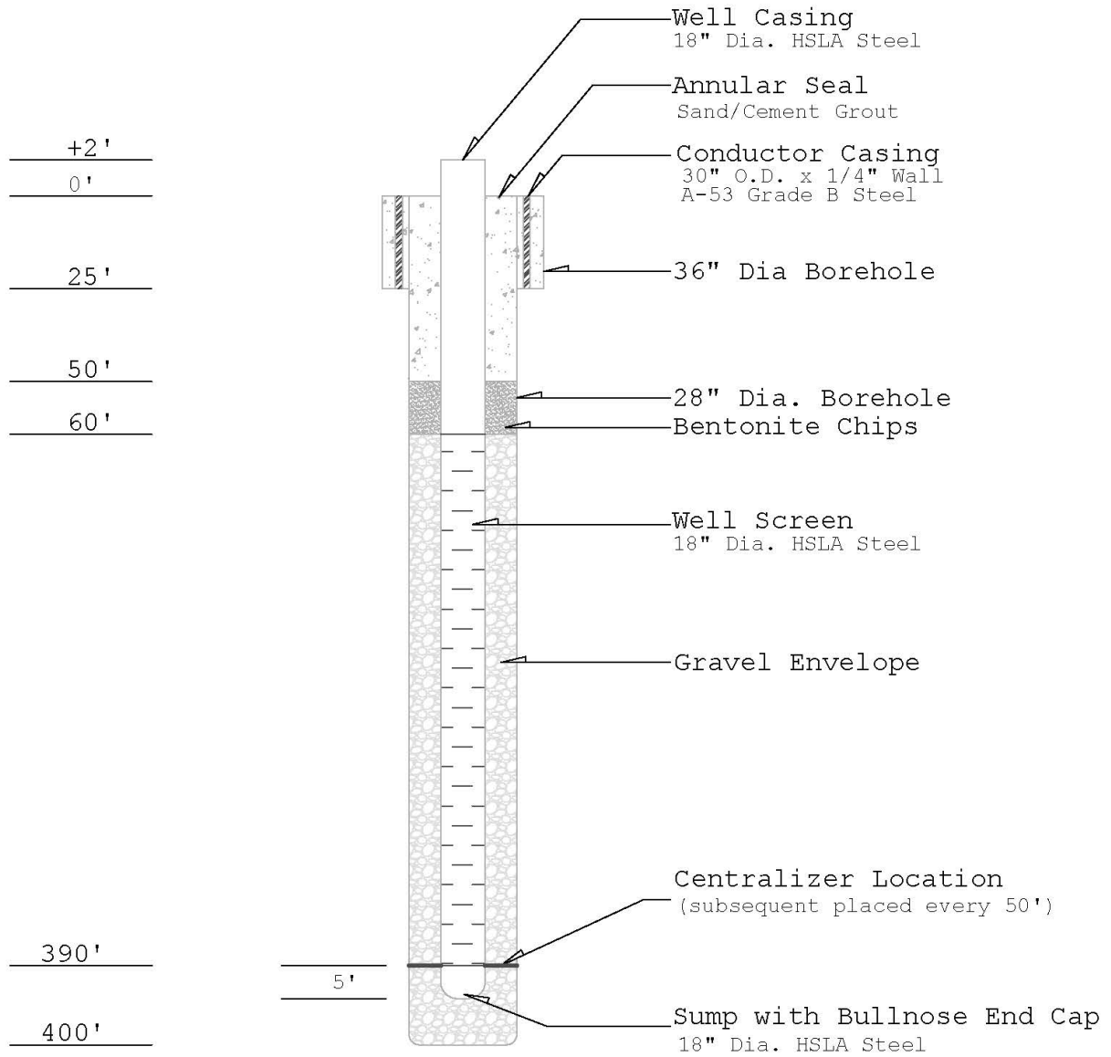
Figure 8 - Preliminary design of W076R, replacement for well W076
