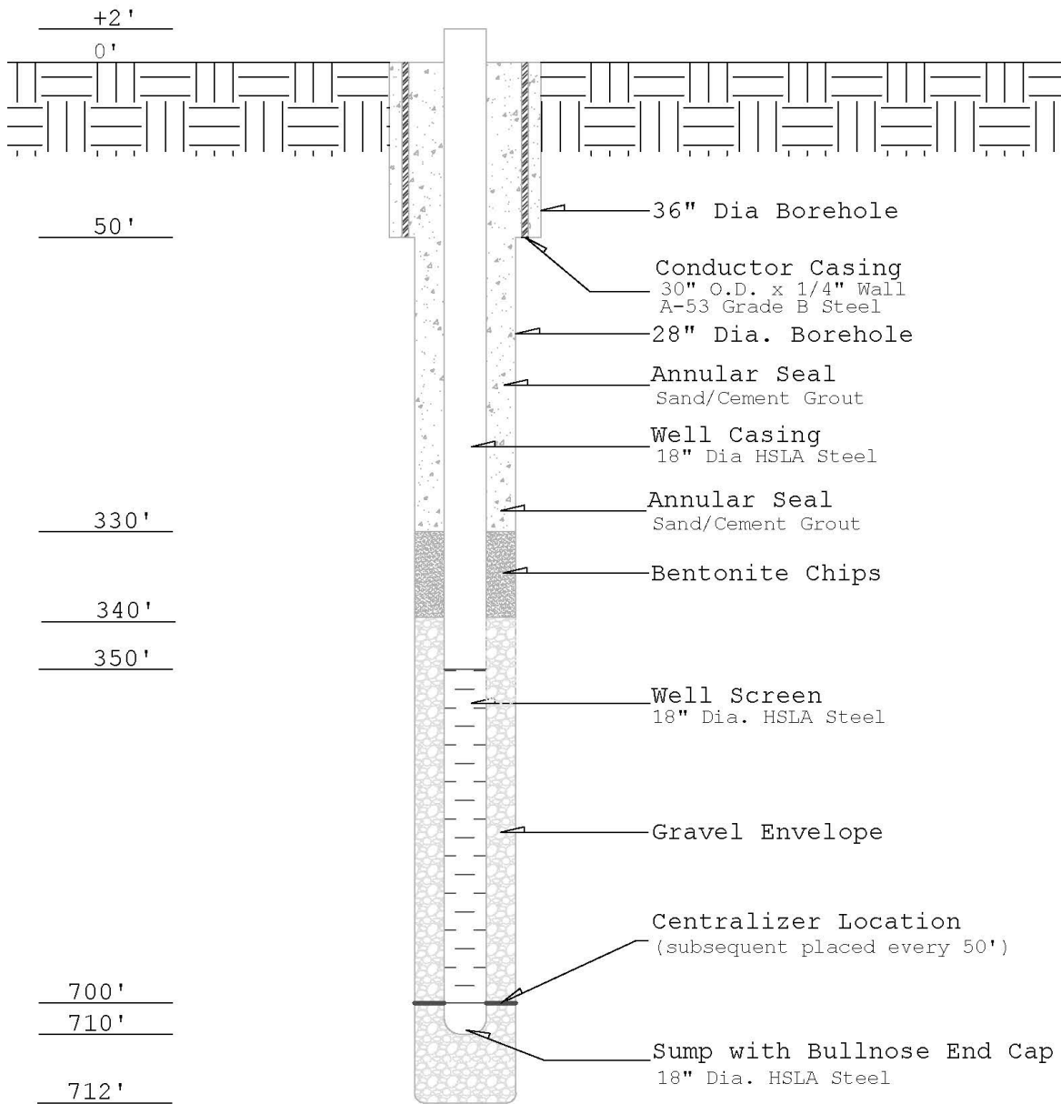
Figure 7 – Preliminary design for W371R in Bishop
