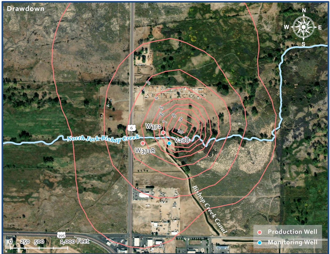
Figure 8 – Drawdown contours of groundwater levels in the shallow aquifer from pumping original W371 at 2.5 cfs for one year
