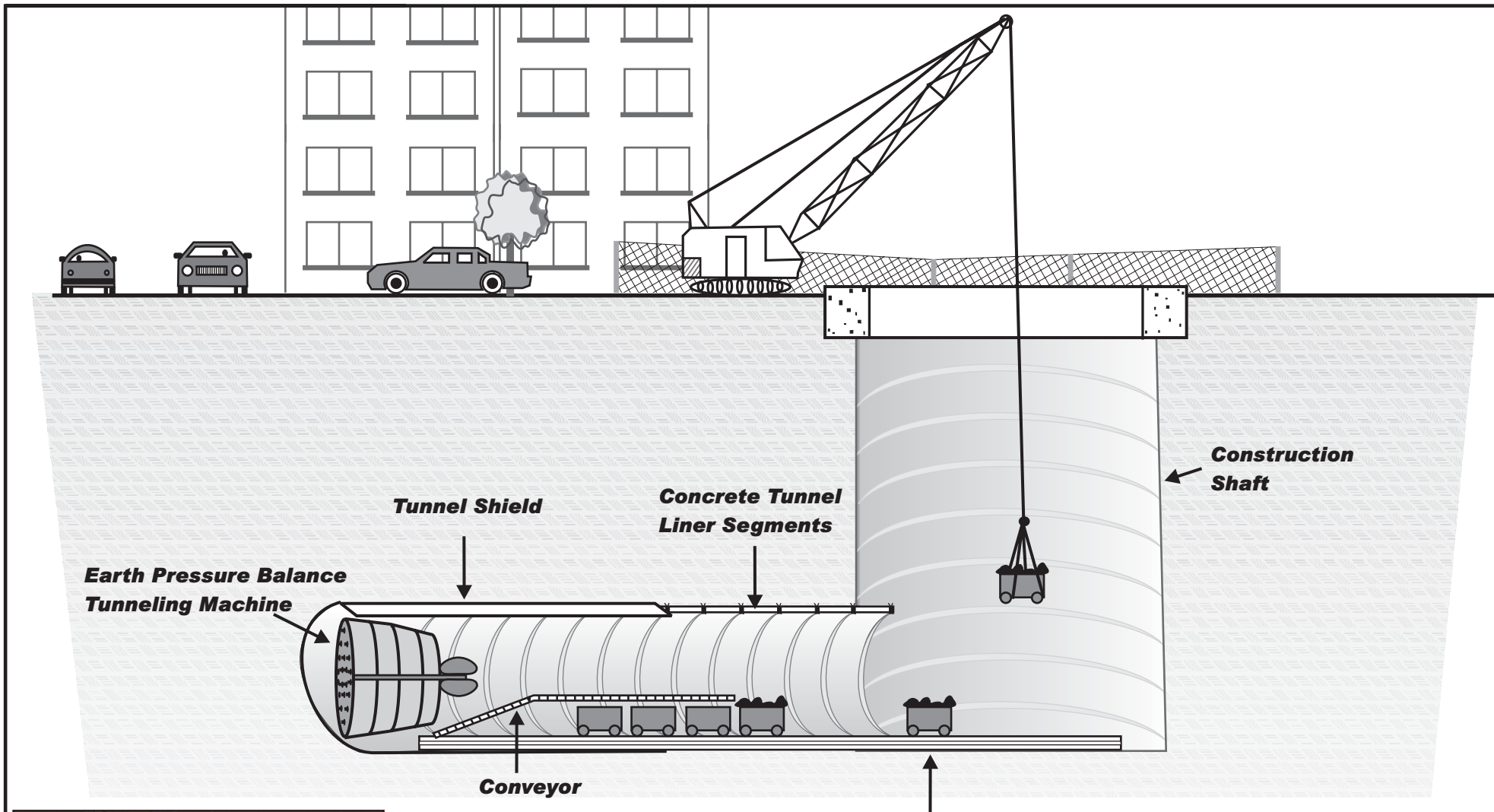
RSCI -- Upper Reach Figure 2-4 Typical Tunneling Operation
